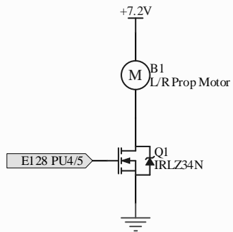
Propeller Motor Drive
